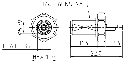
SMA DETAIL DRAWING
